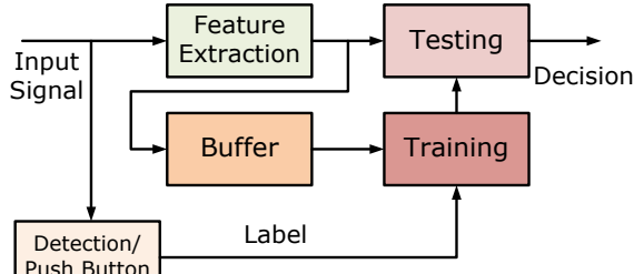
Fig. 3. On-line retraining method. The input data can be labeled by detection/push button input, and the model can be refined through retraining, considering the computing throughput and the variation of EEG data. For example, in our study, a retraining period of half an hour is feasible with SVM training algorithm implemented on a RISC processor.
