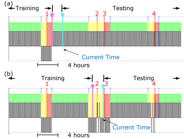
Fig. 10. The two snapshot of patient 11 in Freiburg database. (a) The response of the retrained classifier right after learning the first seizure onset. It shows that the classifier has no prediction ability of the future seizure onsets. (b) The response of the retrained classifier after learning part of preictal data of the second seizure onset. The classifier gains the ability to predict the third and the fourth seizure onsets.
