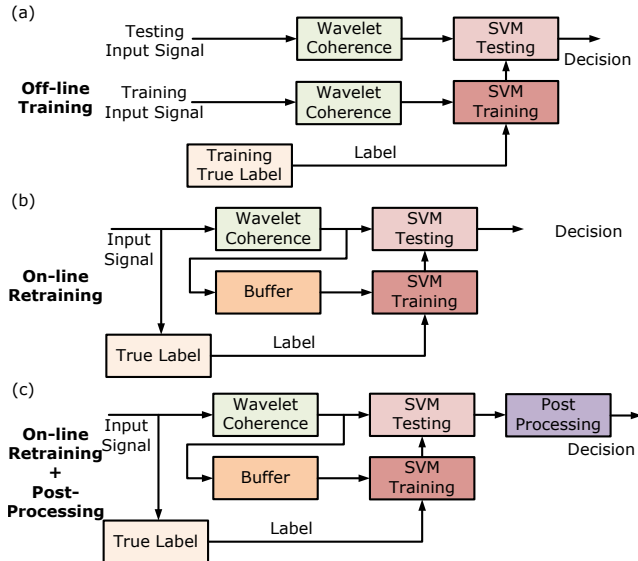
Fig. 6. The algorithm flows. (a) Off-line training method. (b) On-line retraining method. (c) On-line retraining method with post-processing scheme.
